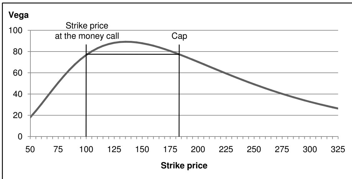
Figure 3: Vega as a function of the strike price.
