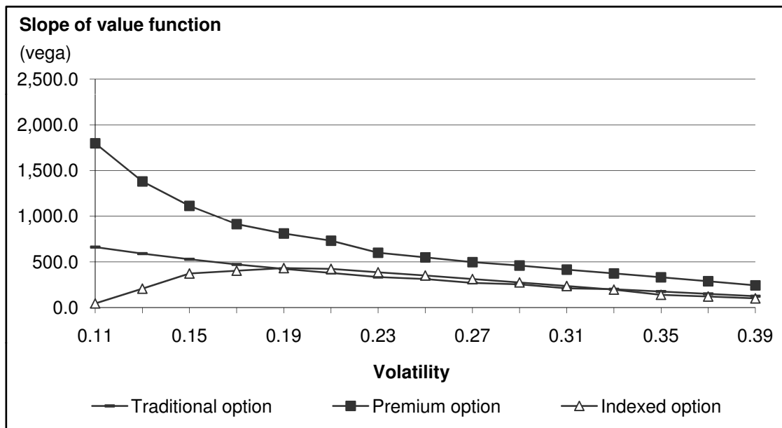
Figure 2: Influence of caps on the vegas of different plan structures.
