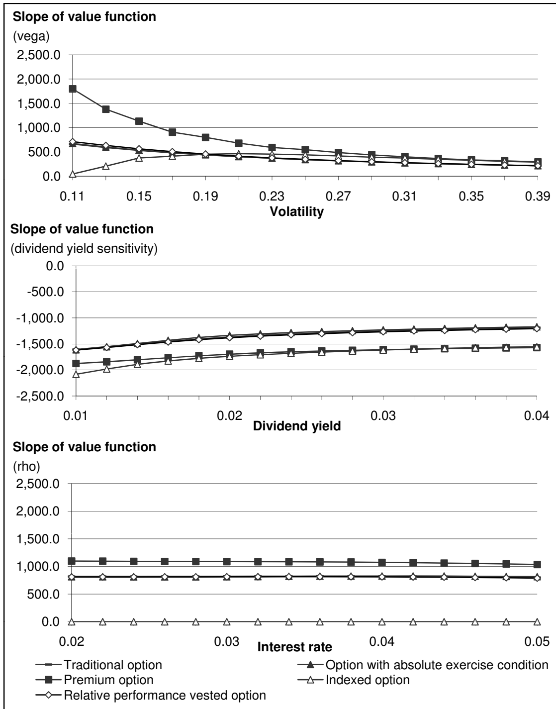
Figure 1: Slopes of the plans' value functions with respect to volatility, dividend yield, and interest rate.
